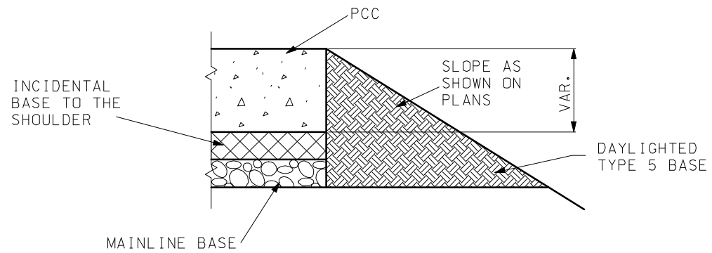
PCC PAVEMENT
