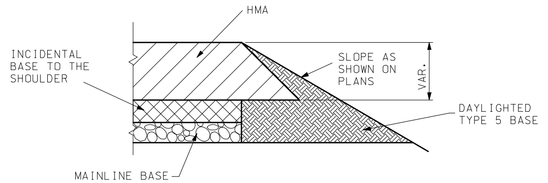
HMA PAVEMENT
